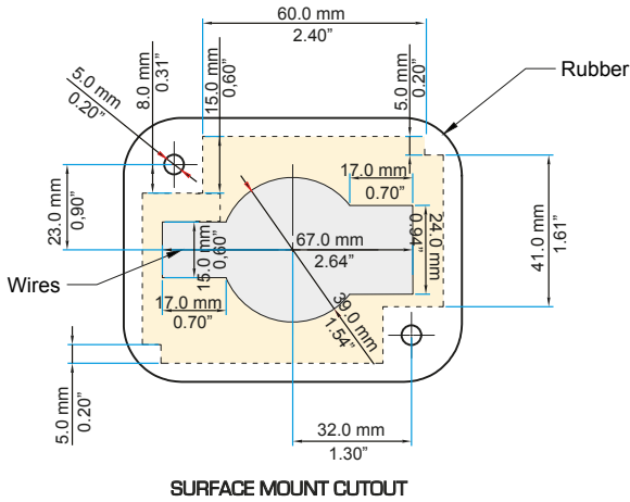
SURFACE MOUNT CUTOUT
